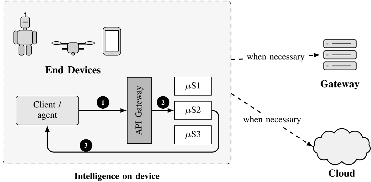
Fig. 3. DFC-AI. The API gateway and microservices run on the end device: (1) the client invokes the local API gateway, (2) the gateway dispatches to a local microservice, (3) the result returns. Dashed arrows show optional escalation to a gateway or the cloud.
