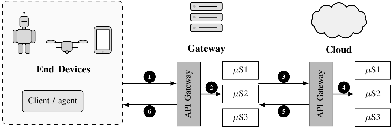
Fig. 2. Gateway-based edge AI. (1) device offloads to the gateway; (2) gateway dispatches internally; (3) gateway escalates to the cloud when needed; (4) cloud dispatches internally; (5)–(6) results return via the gateway.
