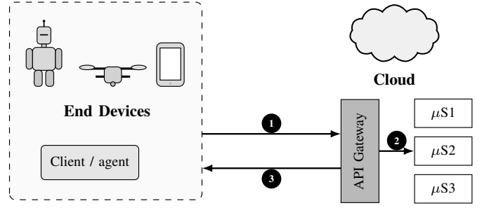
Fig. 1. Centralized cloud AI. (1) the device sends raw context to the cloud; (2) the application programming interface (API) gateway dispatches to the microservices; (3) the result returns.
