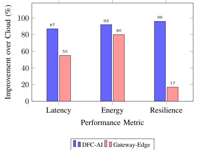
Fig. 4. Improvement over cloud in latency, energy, and resilience, averaged across scenarios (%)
