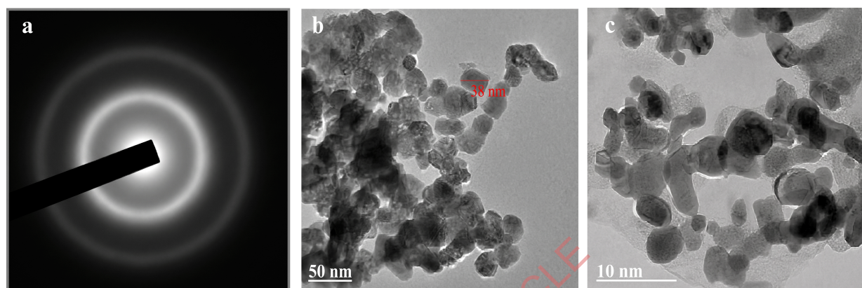
Figure 5: HR-TEM analysis of CA 4 -ZnO nanocomposite hydrogels.
