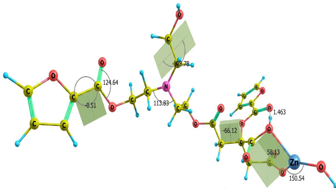
Figure 14: The optimized geometry of the CA 4 -ZnO nanocomposite hydrogels.
