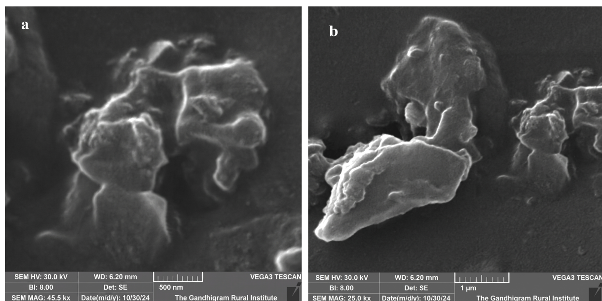
Figure 3: SEM analysis of [CA 4 -ZnO] nanocomposite hydrogels of CA 4 Z 3 .
