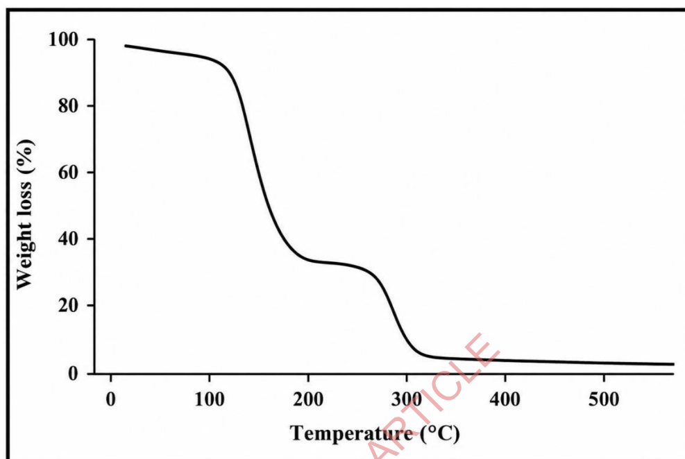
Figure 6: TGA of [CA 4 -ZnO] nanocomposite hydrogels.
