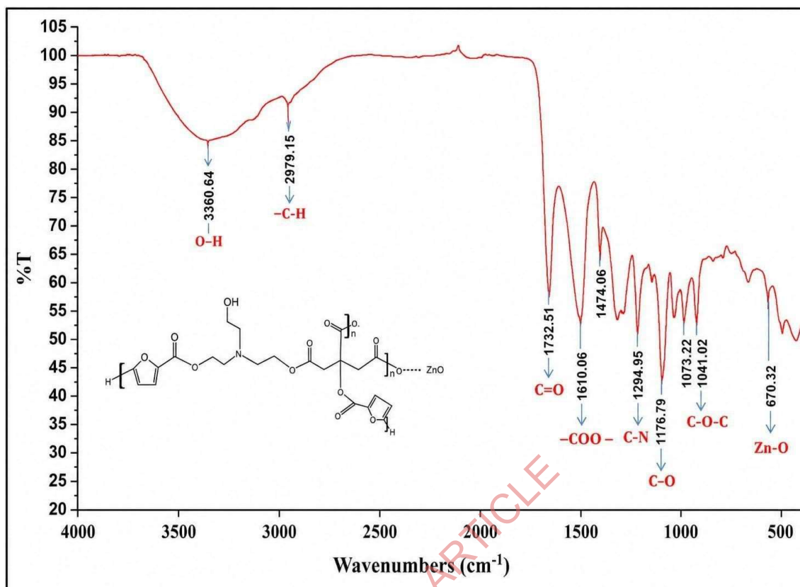
Figure 1: FTIR spectrum of CA 4 -ZnO nanocomposite hydrogels.
