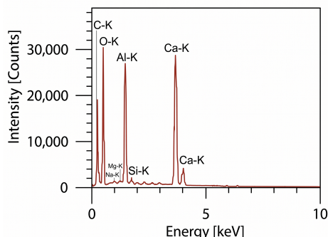
Figure 4: Spectra of modified calcite.
