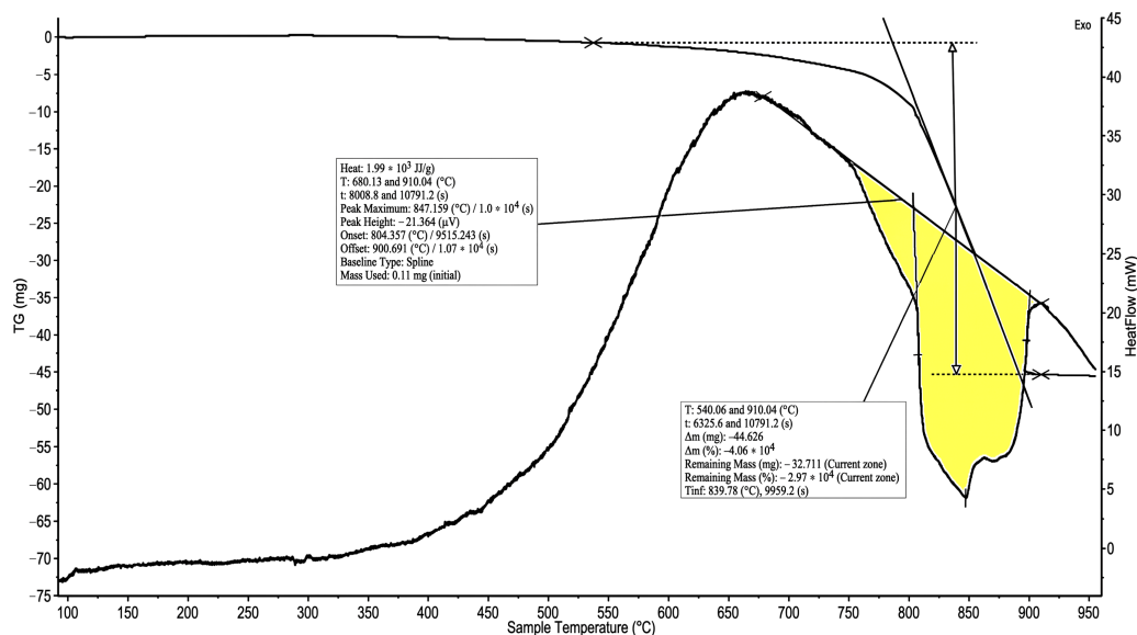
Figure 2: Thermal curves of calcite-limestone.
