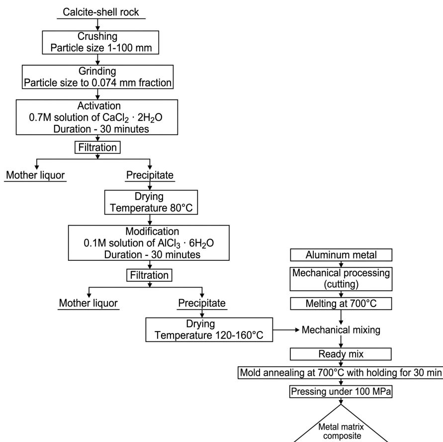
Figure 5: Technological scheme for obtaining a metal-matrix composite material based on calcite shell rock.
