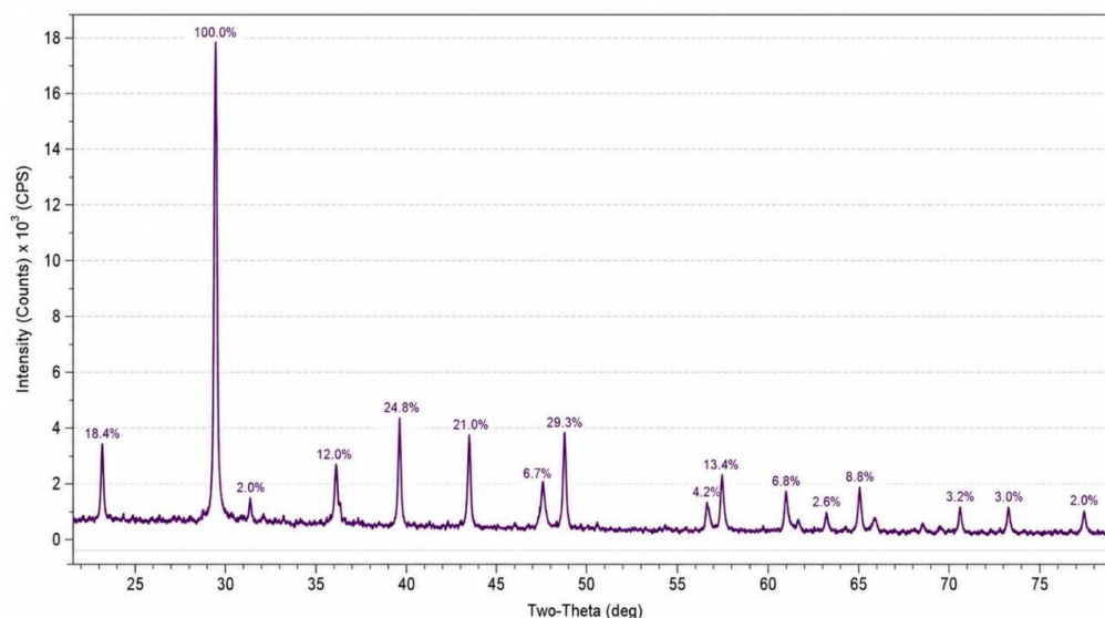
Figure 1: X-ray diffraction pattern of calcite shell rock.
