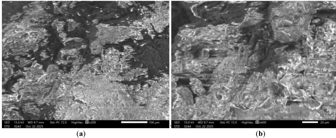
Figure 6: Microstructure of the aluminum-matrix composite at (a) \times 200 and (b) \times 600 magnification.
